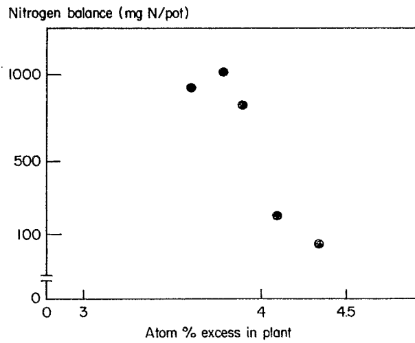
Fig. 2. Relationship between nitrogen balance in flooded soil-rice ecosystem and ^{15}\text{N} content in rice plants.
